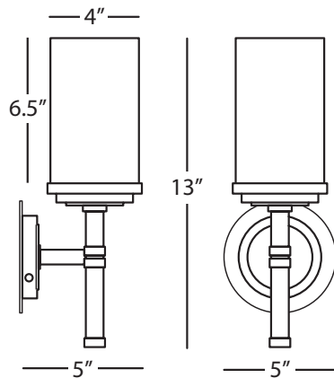
Shown with Optional Junction Box Cover Plate
